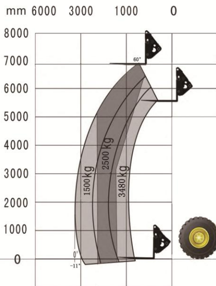
HNT35-4 Load Chart
